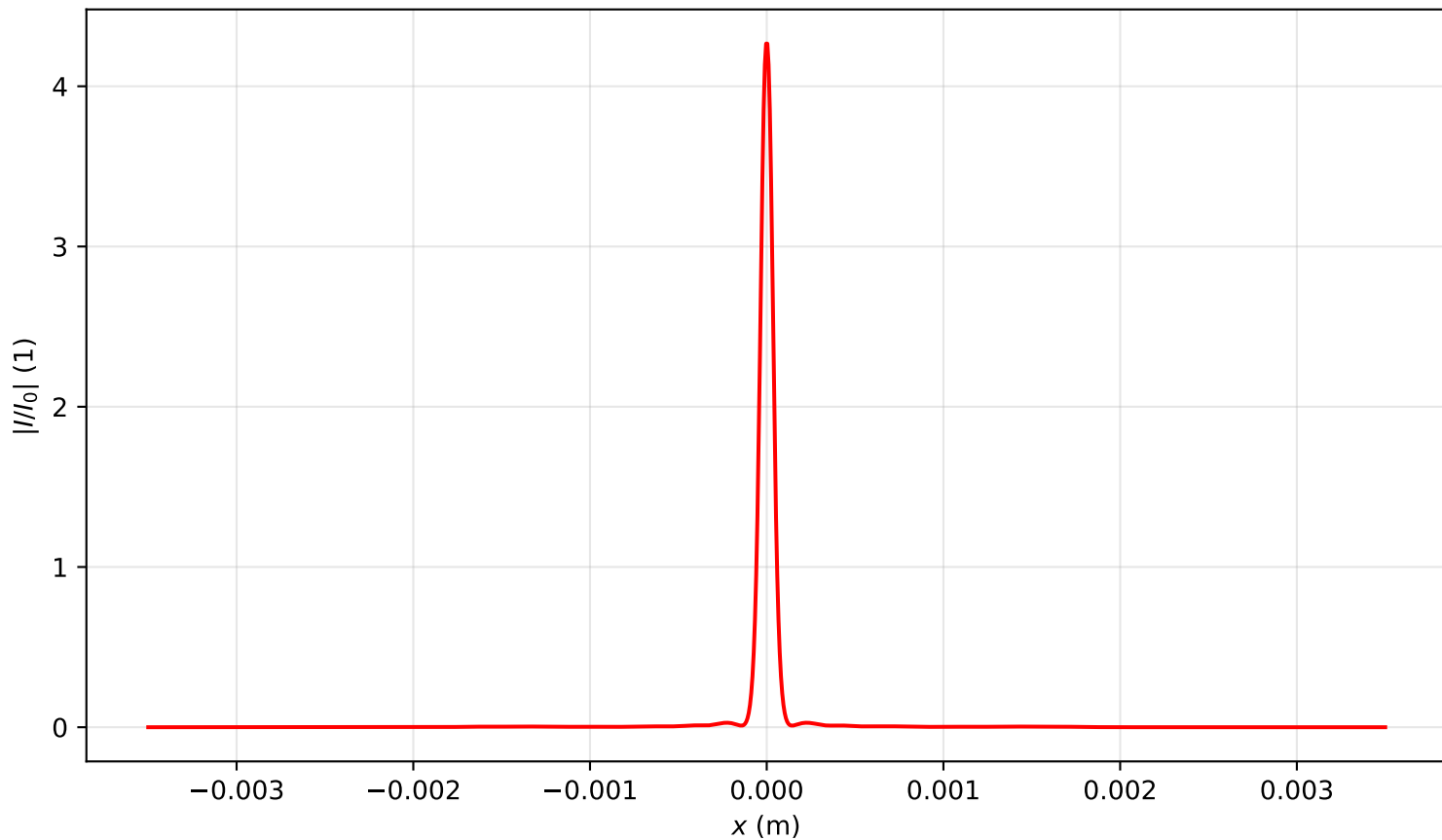
Intensity profile I(x, y = 0, z = 1.911)/I_0 , P_{in}=15.0P_{cr} , artificial time
