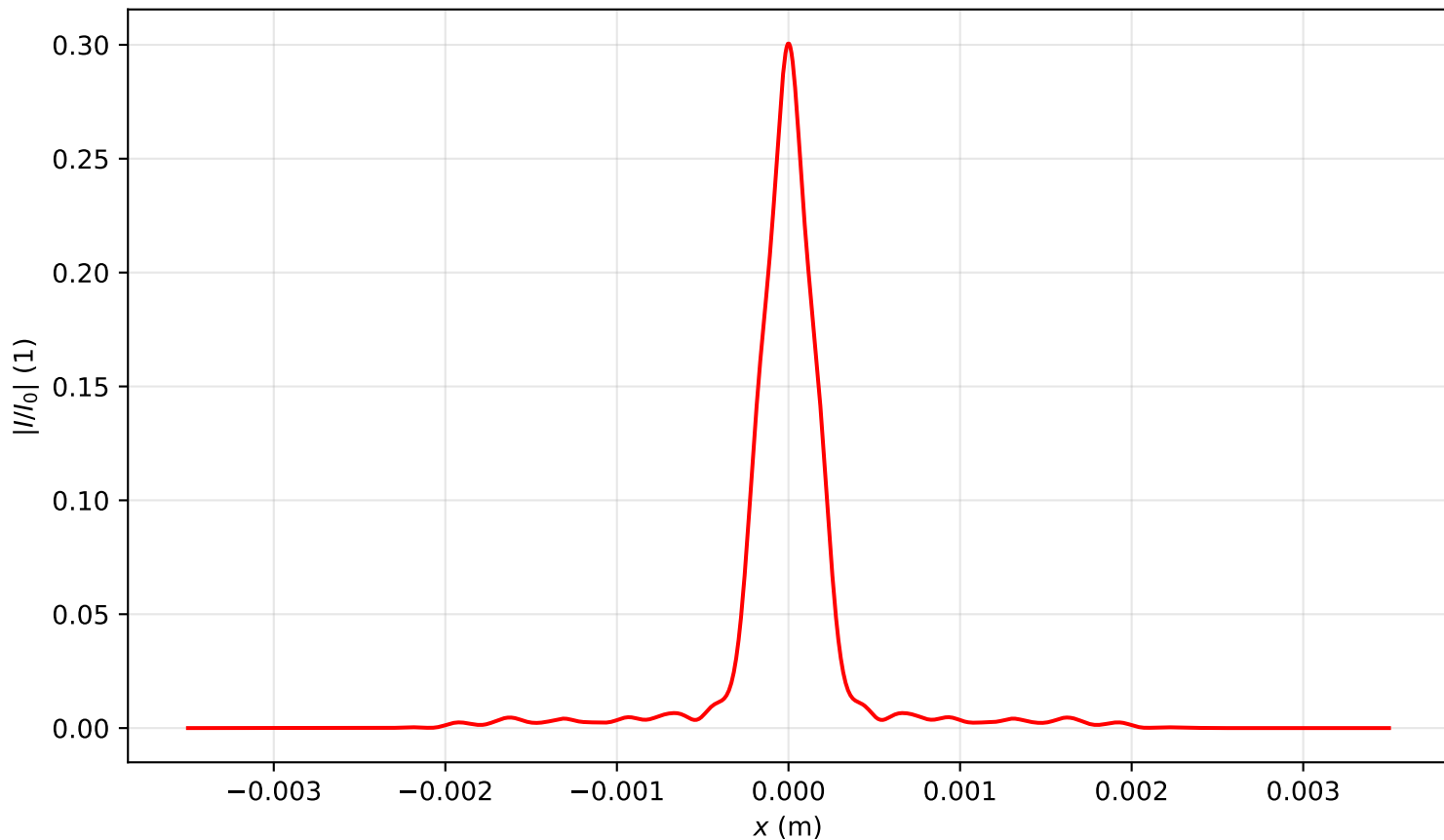
Intensity profile I(x, y = 0, z = 2.070)/I_0 , P_{in}=15.0P_{cr} , artificial time
