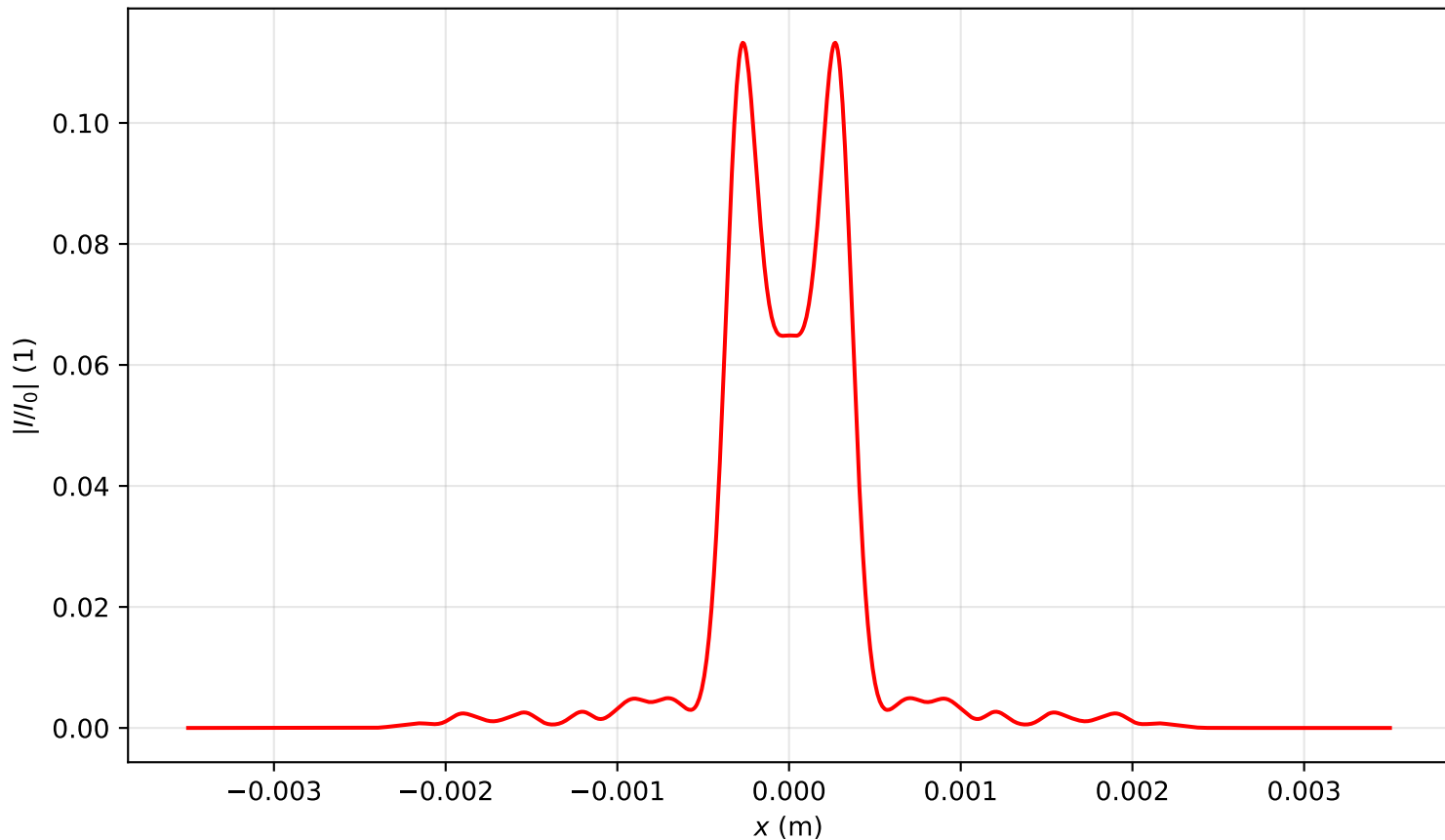
Intensity profile I(x, y = 0, z = 2.229)/I_0 , P_{in}=15.0P_{cr} , artificial time
