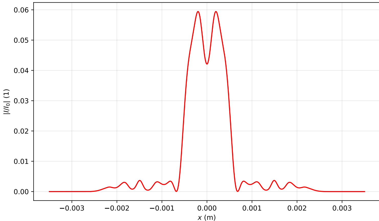
Intensity profile I(x, y = 0, z = 2.388)/I_0 , P_{in}=15.0\text{Pcr} , artificial time
