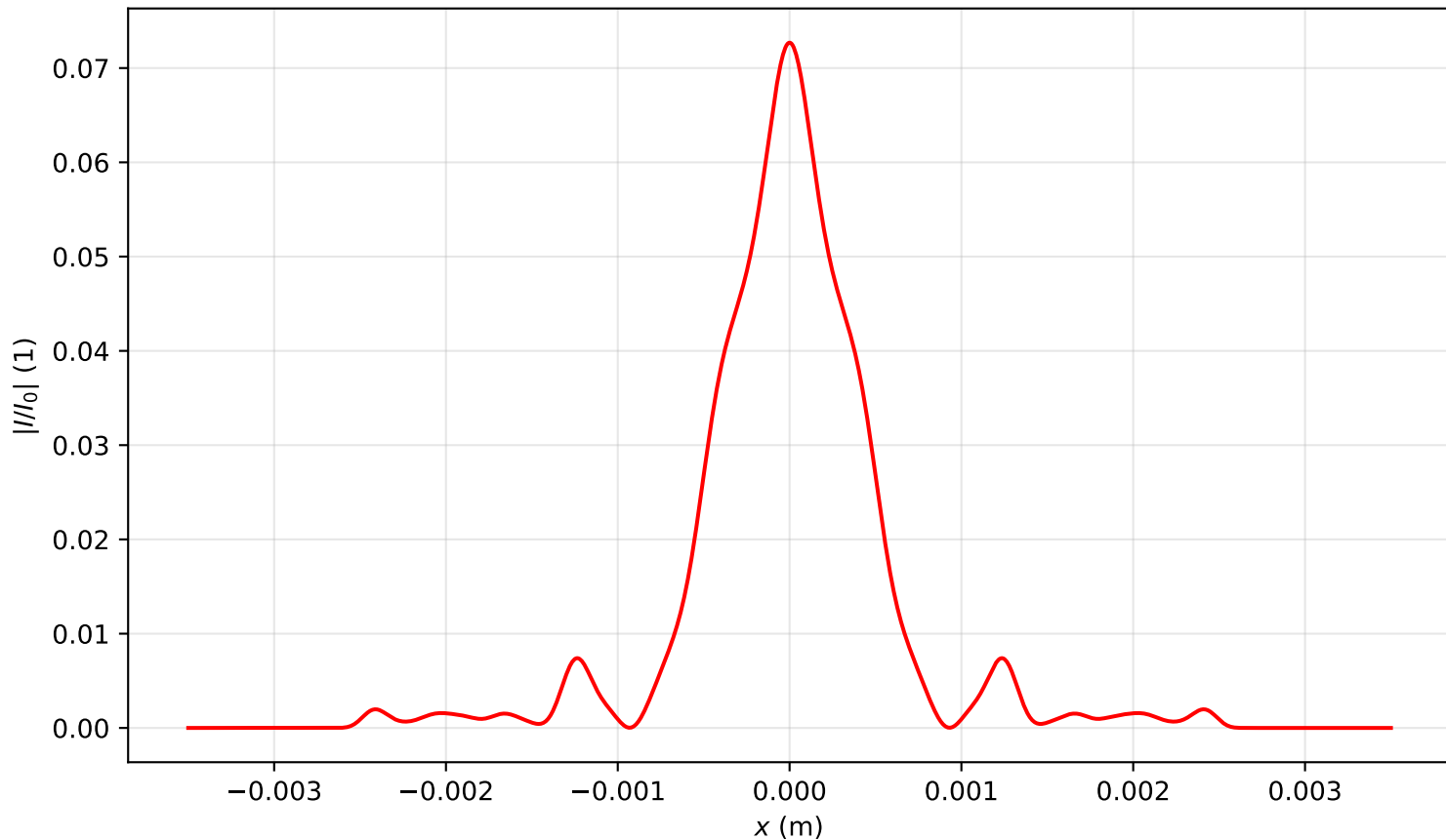
Intensity profile I(x, y = 0, z = 2.707)/I_0 , P_{in}=15.0P_{cr} , artificial time
