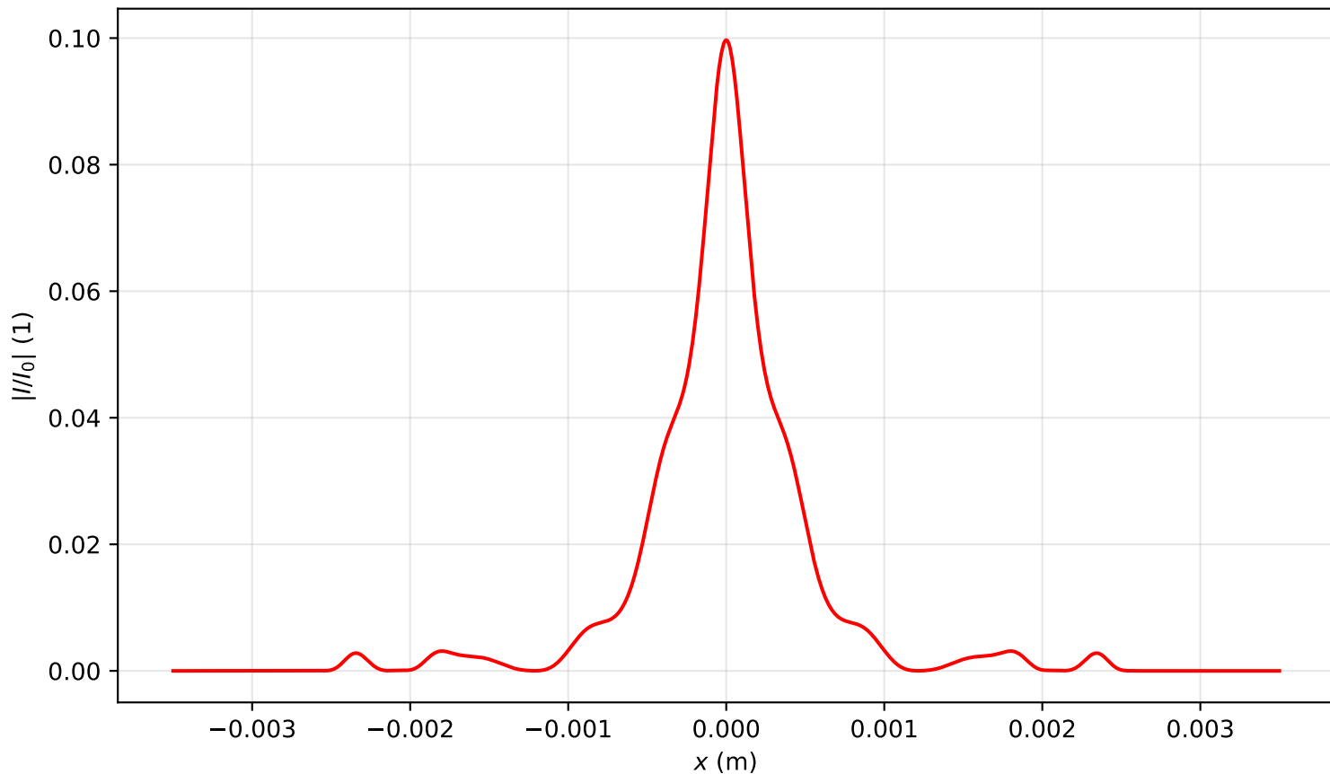
Intensity profile I(x, y = 0, z = 3.184)/I_0 , P_{in}=15.0P_{cr} , artificial time
