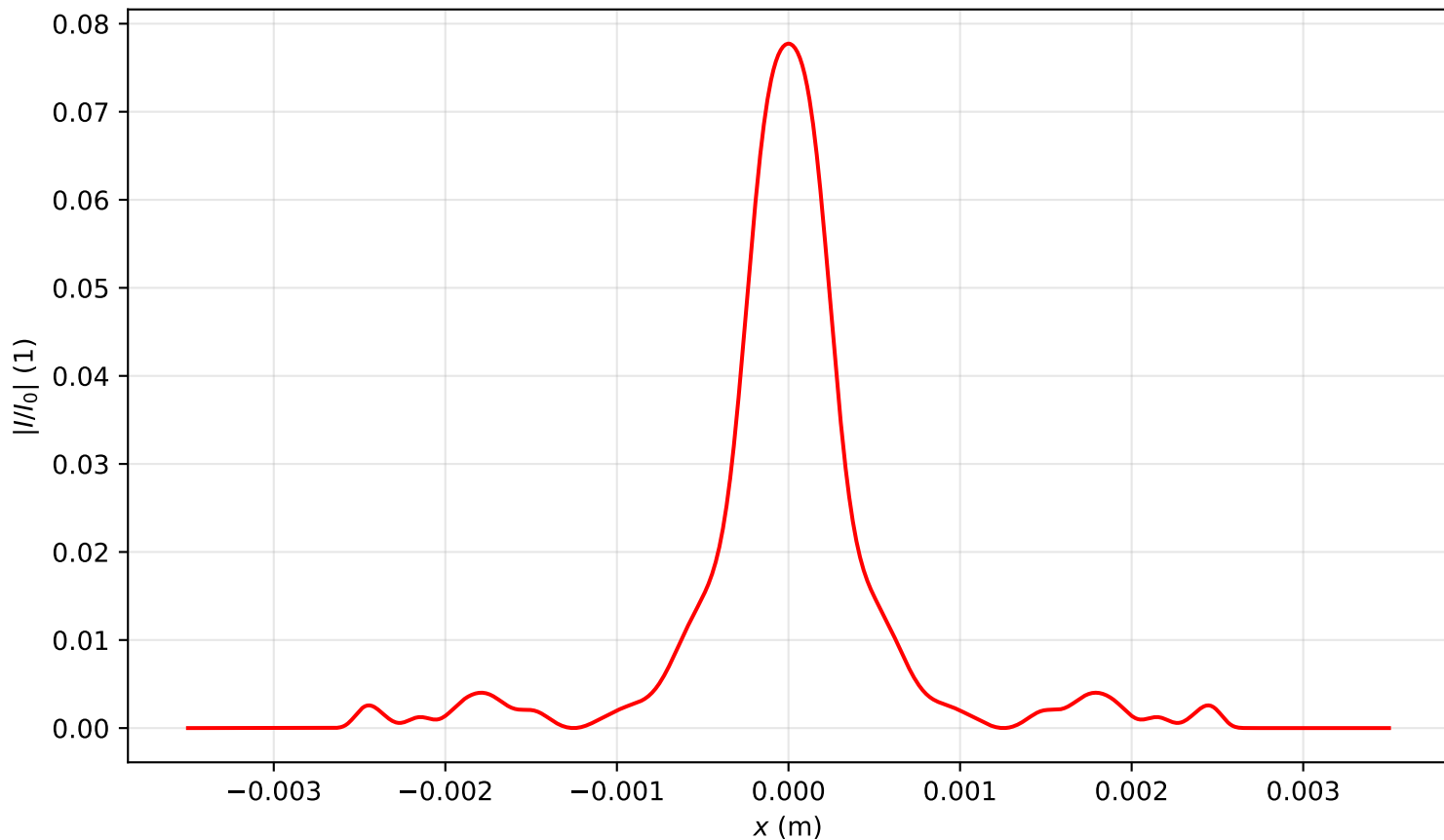
Intensity profile I(x, y = 0, z = 3.344)/I_0 , P_{in}=15.0P_{cr} , artificial time
