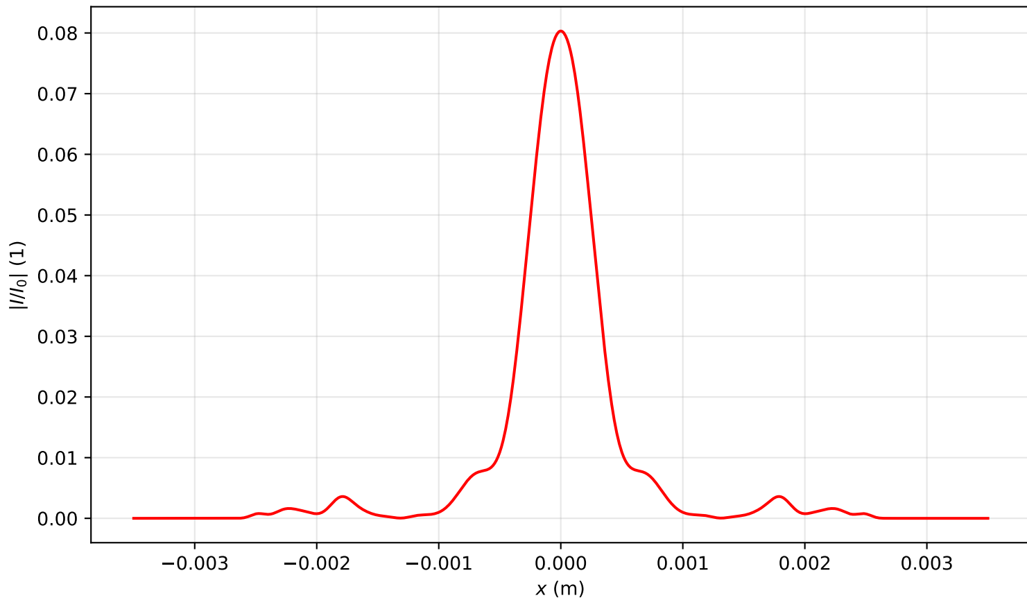
Intensity profile I(x, y = 0, z = 3.503)/I_0 , P_{in}=15.0P_{cr} , artificial time
