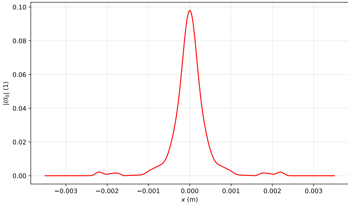
Intensity profile I(x, y = 0, z = 3.662)/I_0 , P_{in}=15.0P_{cr} , artificial time
