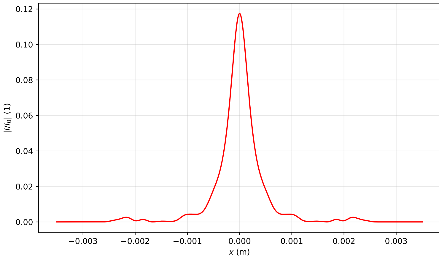
Intensity profile I(x, y = 0, z = 3.821)/I_0 , P_{in}=15.0P_{cr} , artificial time
