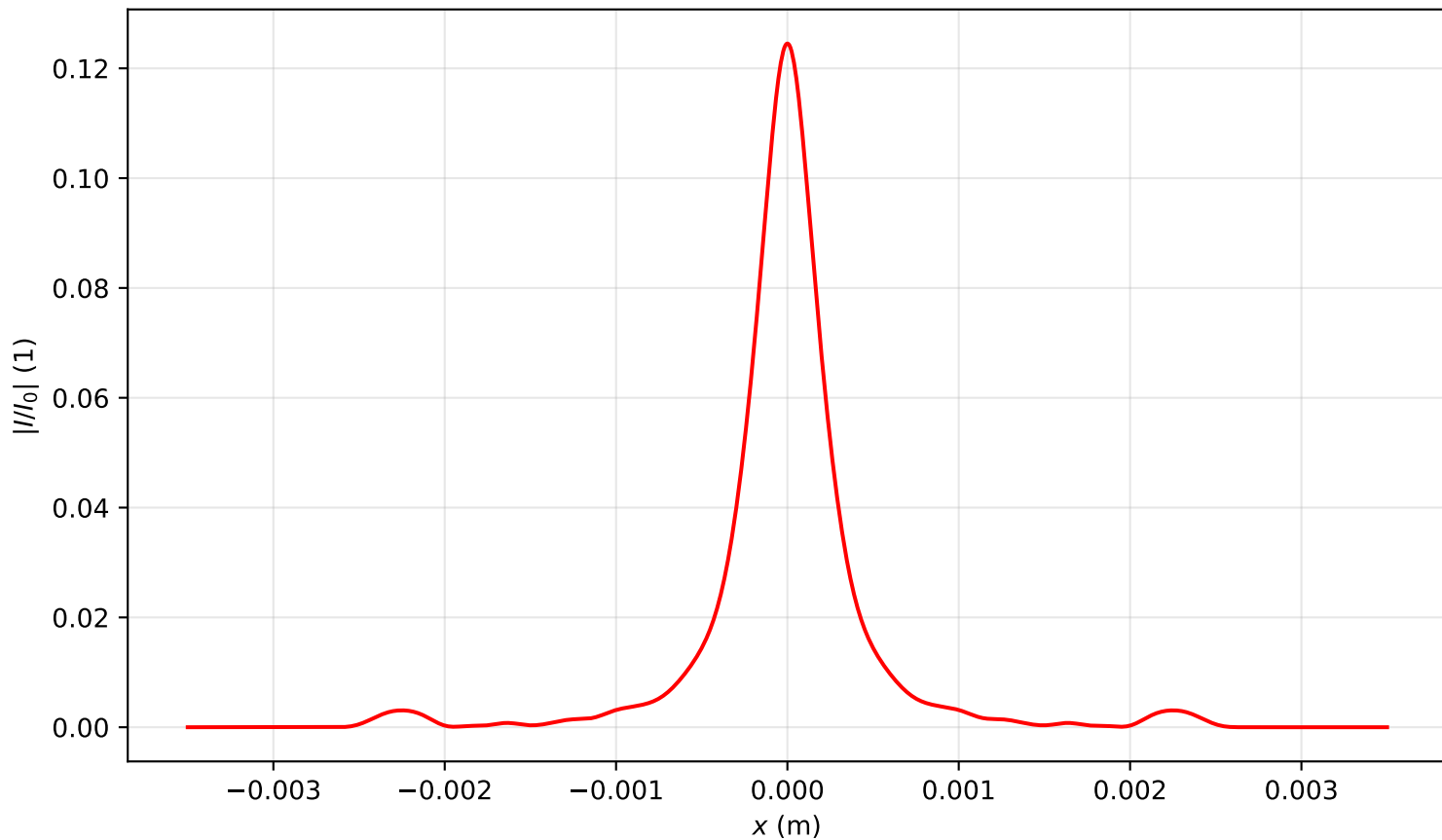
Intensity profile I(x, y = 0, z = 3.981)/I_0 , P_{in}=15.0\text{Pcr} , artificial time
