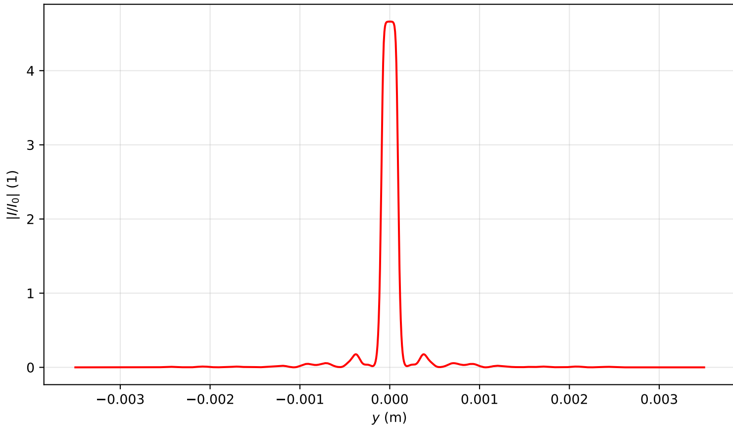
Intensity profile I(x=0, y, z=0.318)/I_0 , P_{in}=15.0P_{cr} , artificial time
