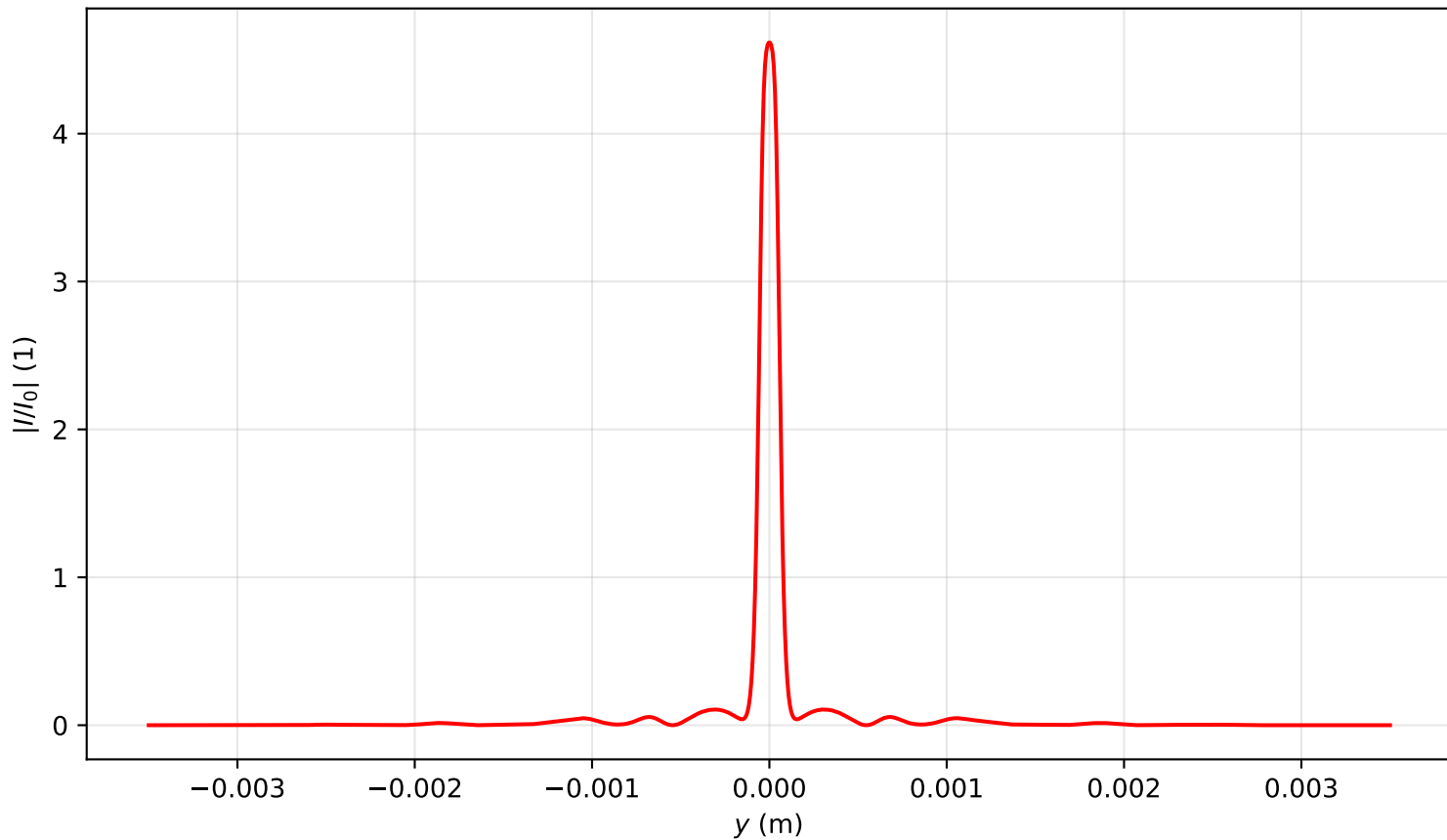
Intensity profile I(x=0, y, z=0.478)/I_0 , P_{in}=15.0P_{cr} , artificial time
