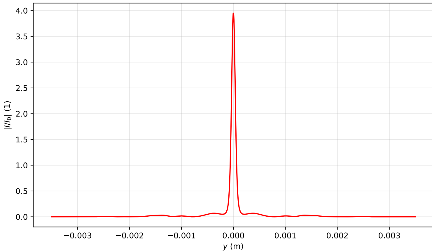
Intensity profile I(x=0, y, z=0.637)/I_0 , P_{in}=15.0P_{cr} , artificial time
