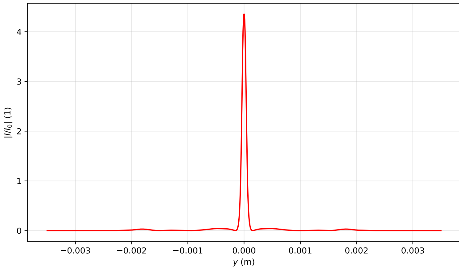
Intensity profile I(x = 0, y, z = 0.796)/I_0 , P_{in}=15.0P_{cr} , artificial time
