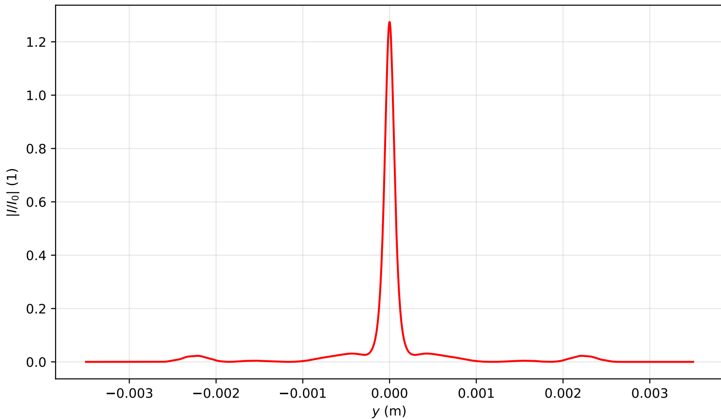
Intensity profile I(x=0, y, z=0.955)/I_0 , P_{in}=15.0P_{cr} , artificial time
