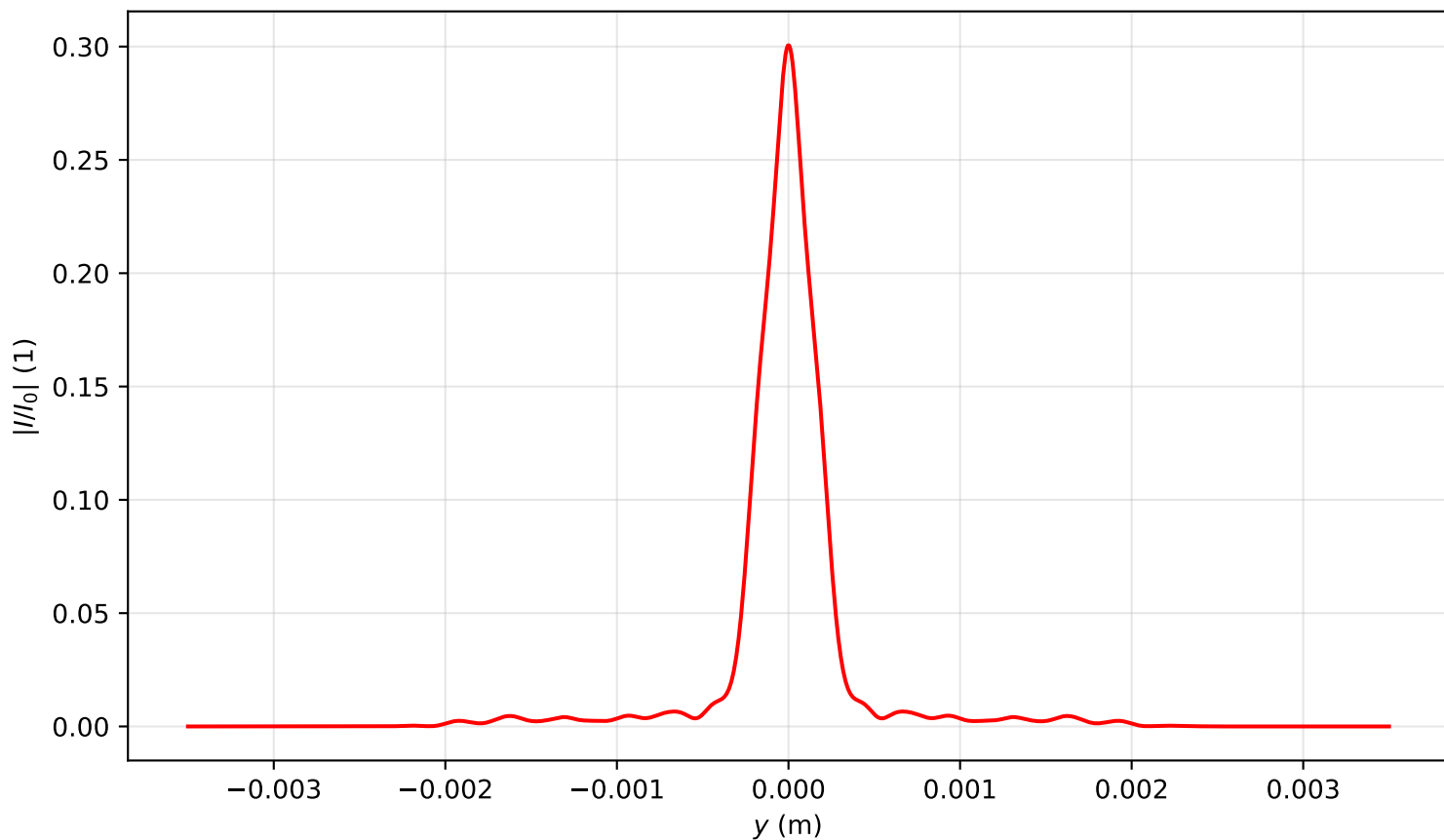
Intensity profile I(x=0, y, z=2.070)/I_0 , P_{in}=15.0P_{cr} , artificial time
