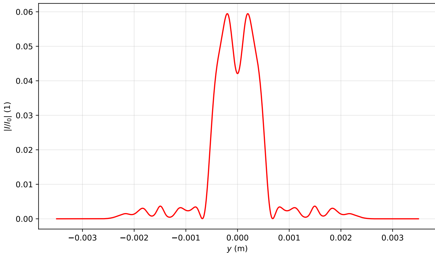
Intensity profile I(x=0, y, z=2.388)/I_0 , P_{in}=15.0\text{Pcr} , artificial time
