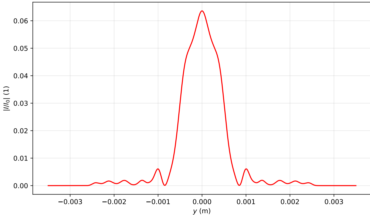
Intensity profile I(x = 0, y, z = 2.548)/I_0 , P_{in}=15.0\text{Pcr} , artificial time
