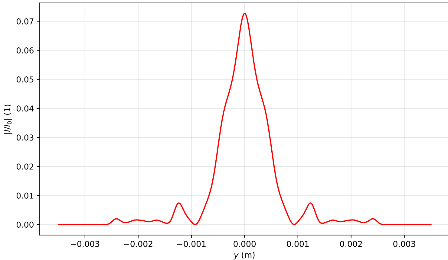
Intensity profile I(x = 0, y, z = 2.707)/I_0 , P_{in}=15.0P_{cr} , artificial time
