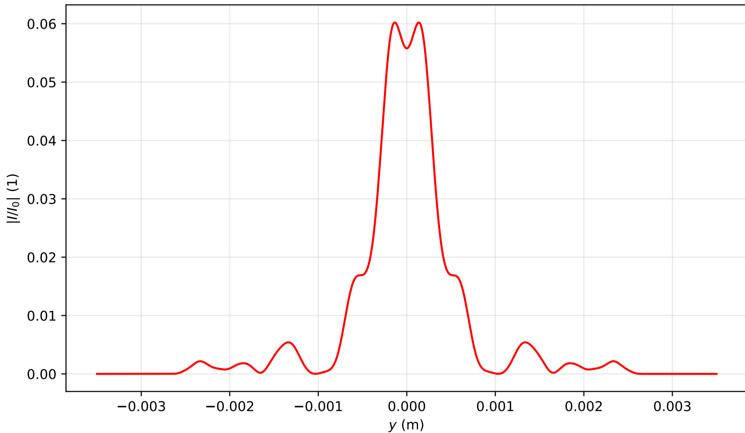
Intensity profile I(x = 0, y, z = 2.866)/I_0 , P_{in}=15.0P_{cr} , artificial time
