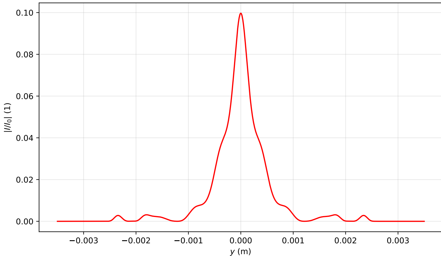
Intensity profile I(x = 0, y, z = 3.184)/I_0 , P_{in}=15.0P_{cr} , artificial time
