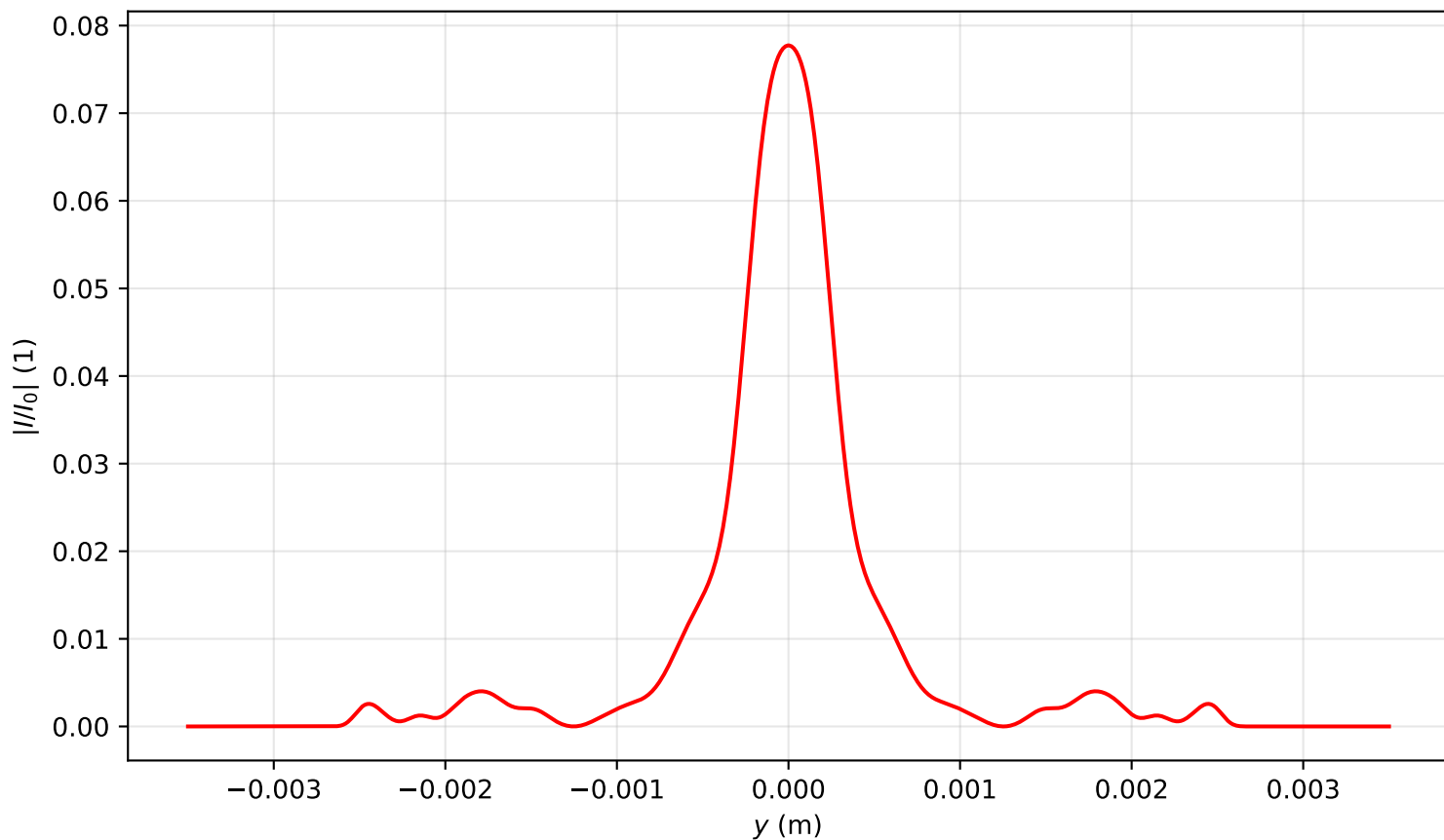
Intensity profile I(x=0, y, z=3.344)/I_0 , P_{in}=15.0P_{cr} , artificial time
