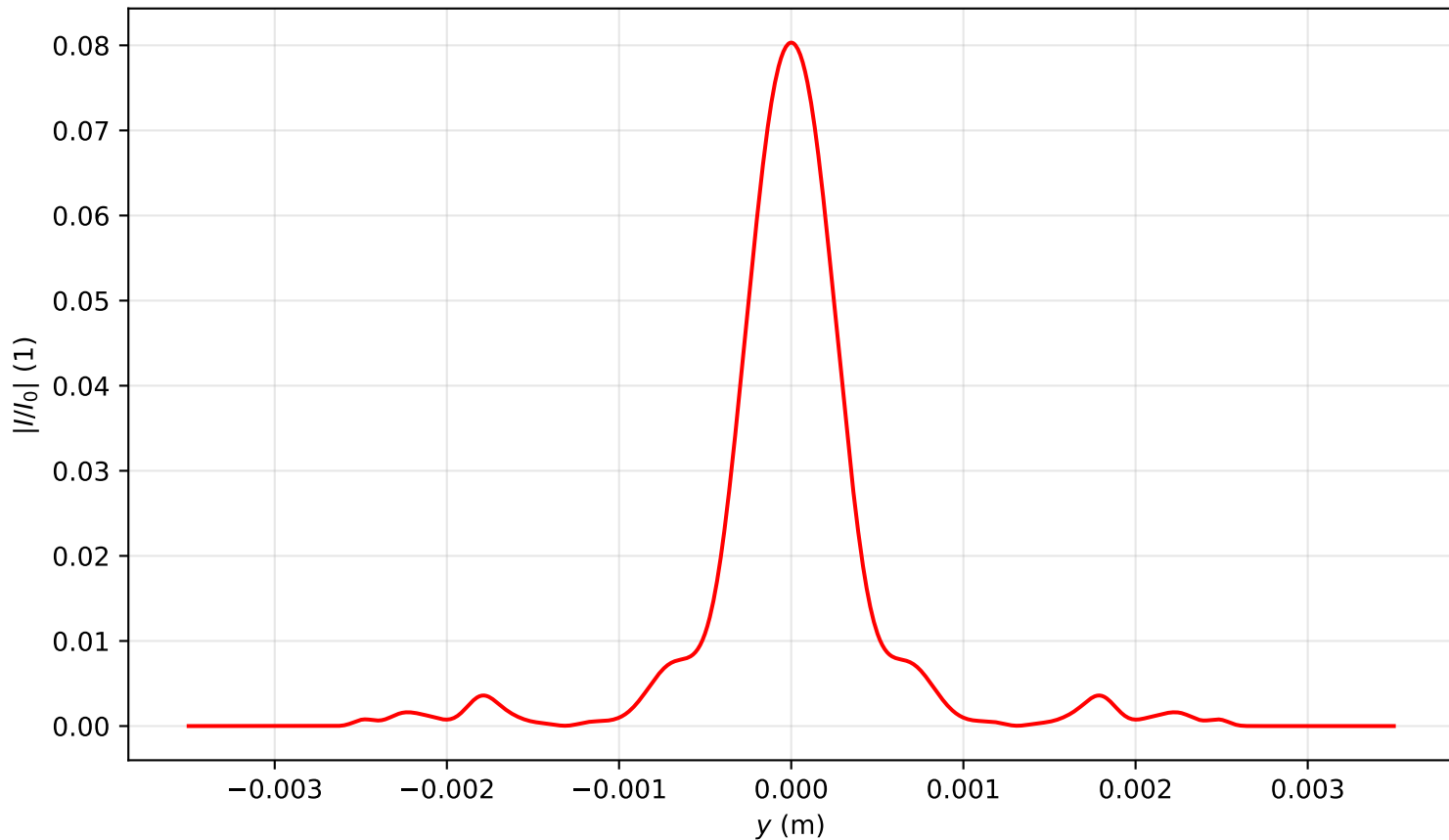
Intensity profile I(x=0, y, z=3.503)/I_0 , P_{in}=15.0P_{cr} , artificial time
