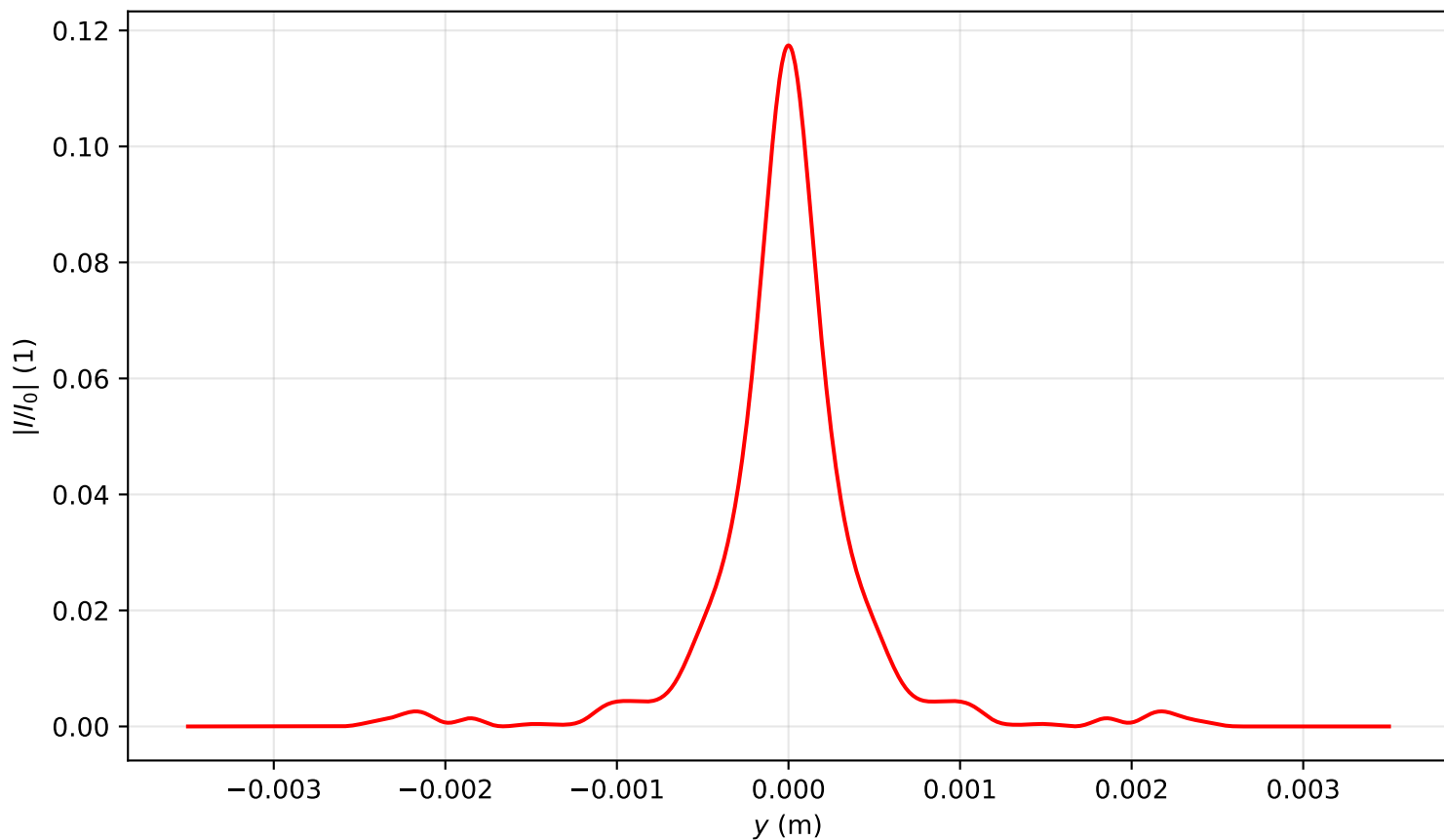
Intensity profile I(x=0, y, z=3.821)/I_0 , P_{in}=15.0P_{cr} , artificial time
