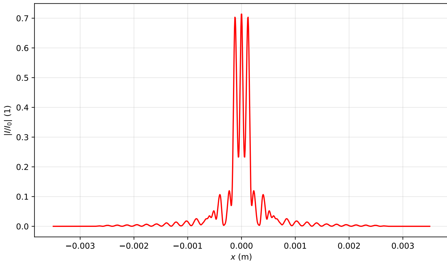
Intensity profile I(x, y = 0, z = 0.159)/I_0 , P_{in}=16.0P_{cr} , artificial time
