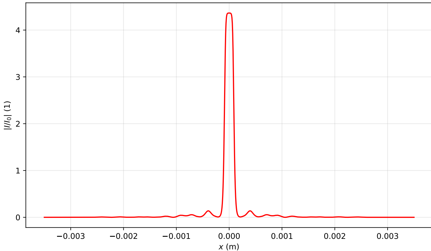
Intensity profile I(x, y = 0, z = 0.318)/I_0 , P_{in}=16.0P_{cr} , artificial time
