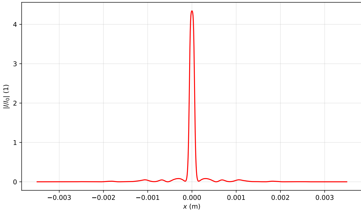
Intensity profile I(x, y = 0, z = 0.478)/I_0 , P_{in}=16.0P_{cr} , artificial time
