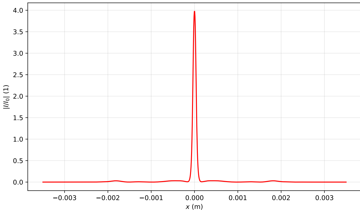
Intensity profile I(x, y = 0, z = 0.796)/I_0 , P_{in}=16.0P_{cr} , artificial time
