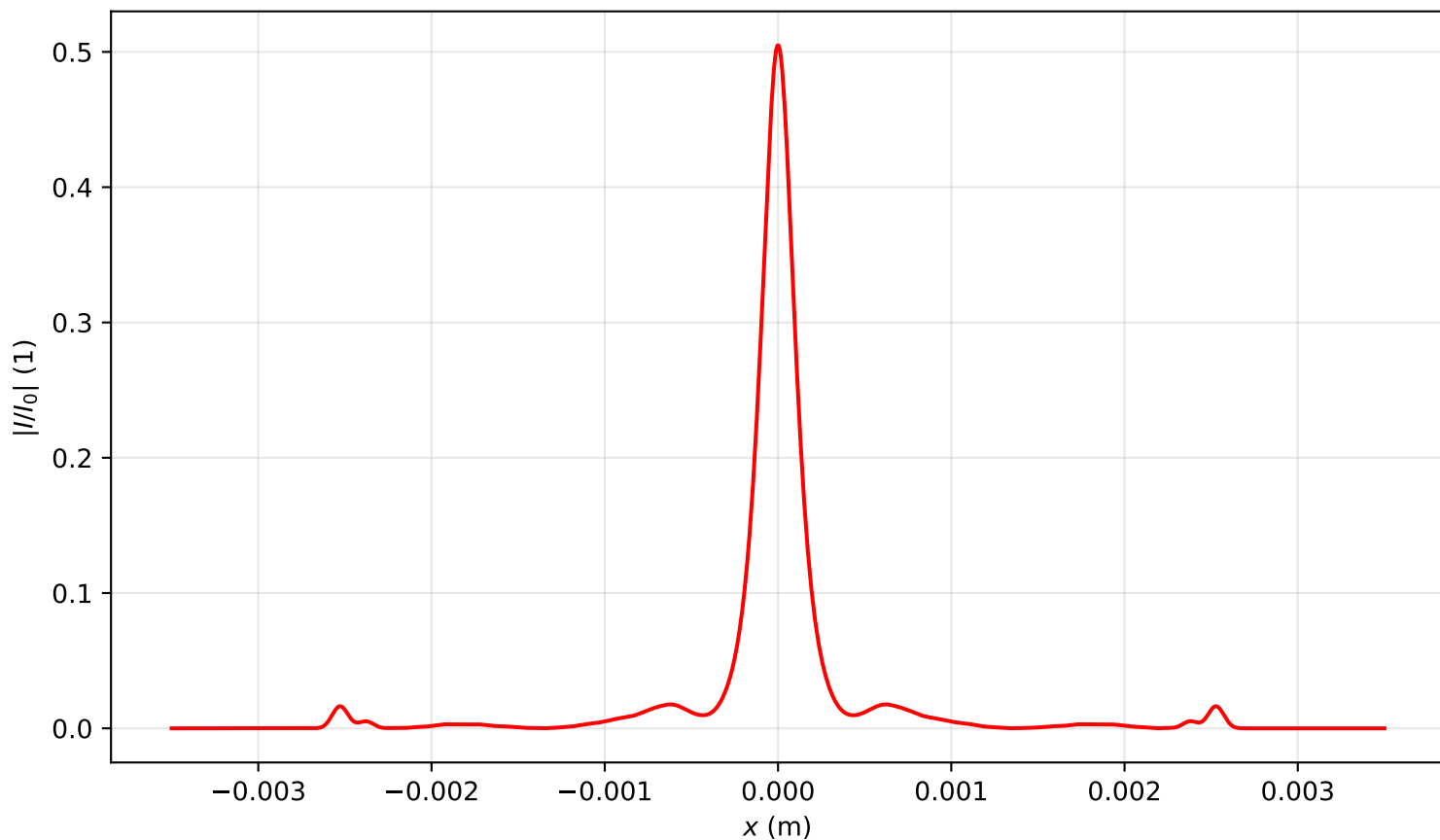
Intensity profile I(x, y = 0, z = 1.115)/I_0 , P_{in}=16.0P_{cr} , artificial time
