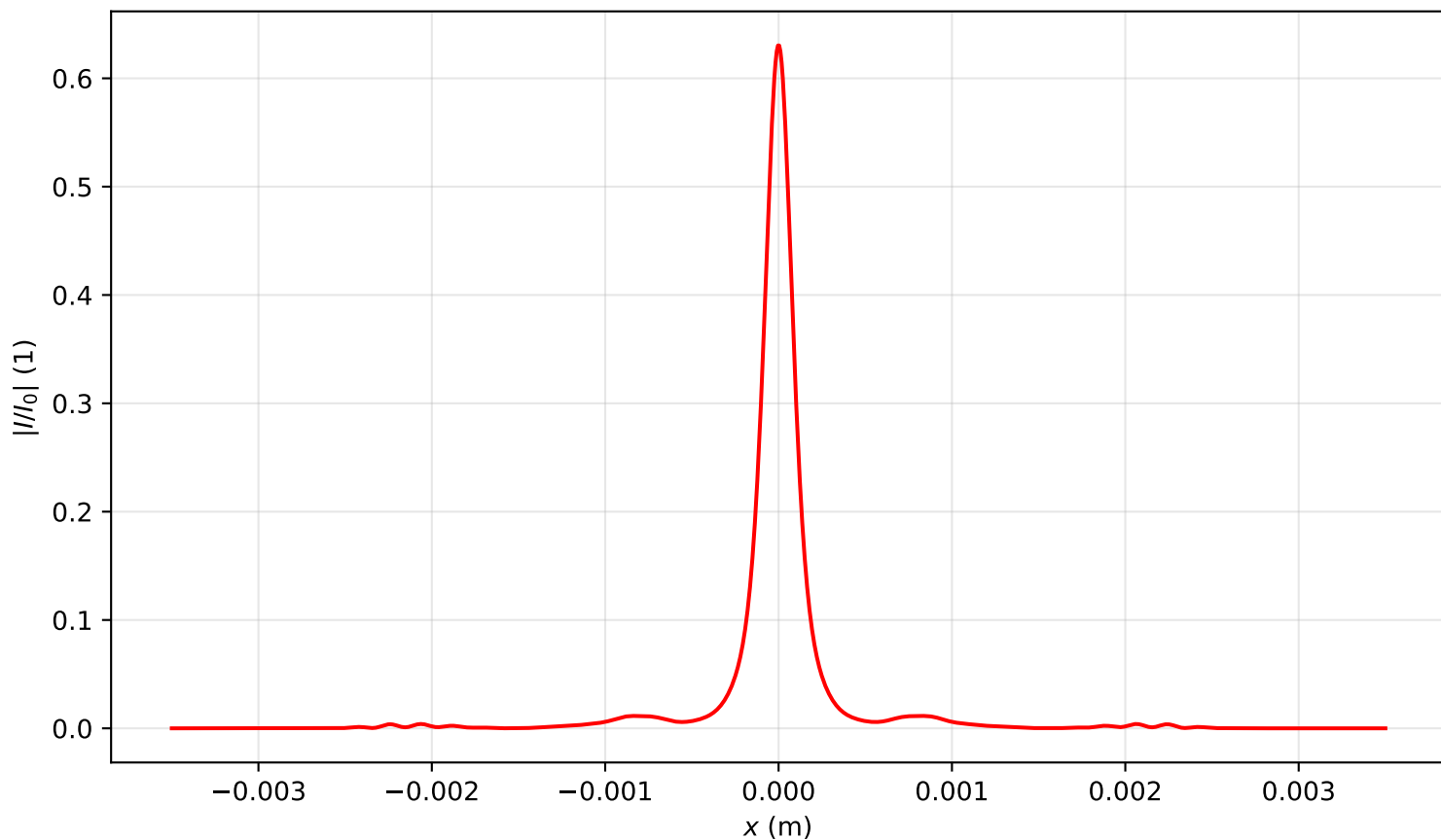
Intensity profile I(x, y = 0, z = 1.274)/I_0 , P_{in}=16.0P_{cr} , artificial time
