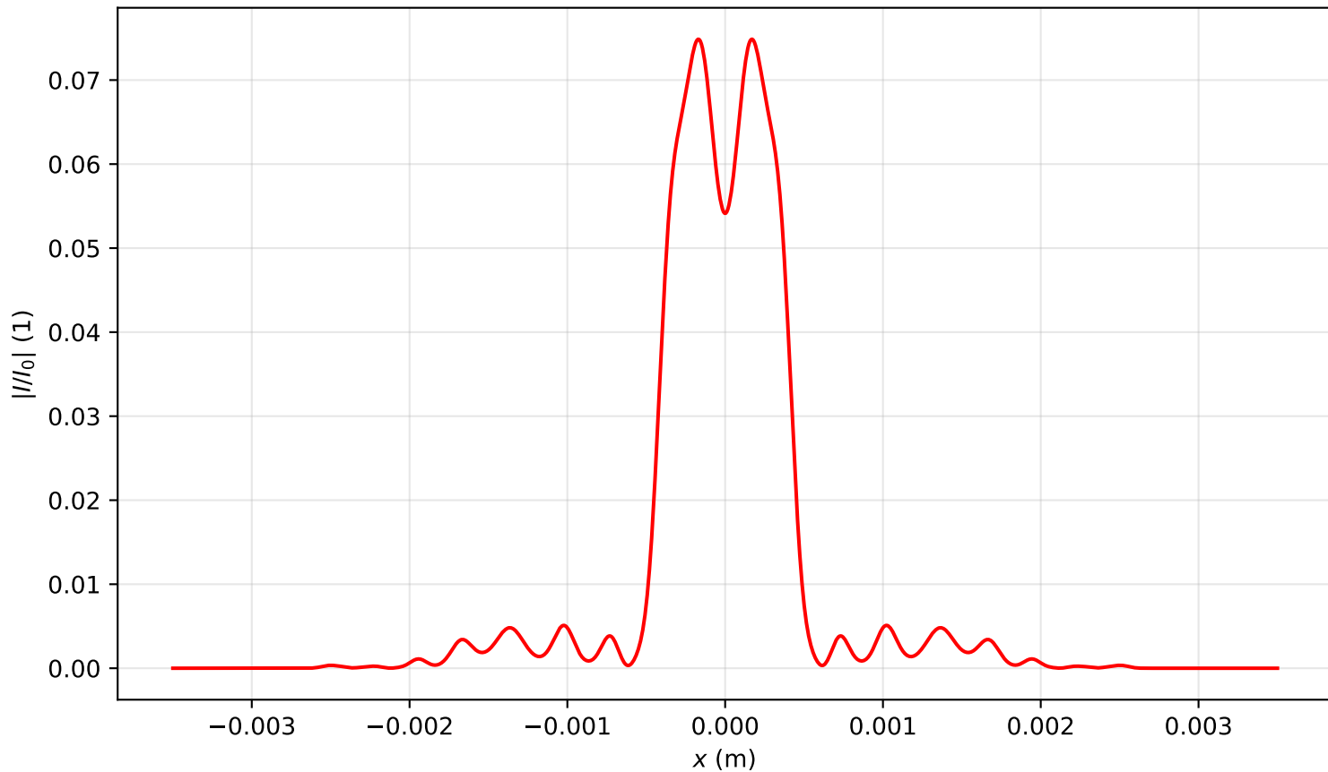
Intensity profile I(x, y = 0, z = 1.911)/I_0 , P_{in}=16.0P_{cr} , artificial time
