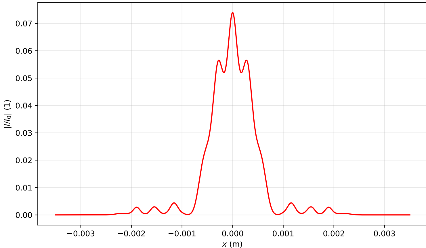
Intensity profile I(x, y = 0, z = 2.229)/I_0 , P_{in}=16.0P_{cr} , artificial time
