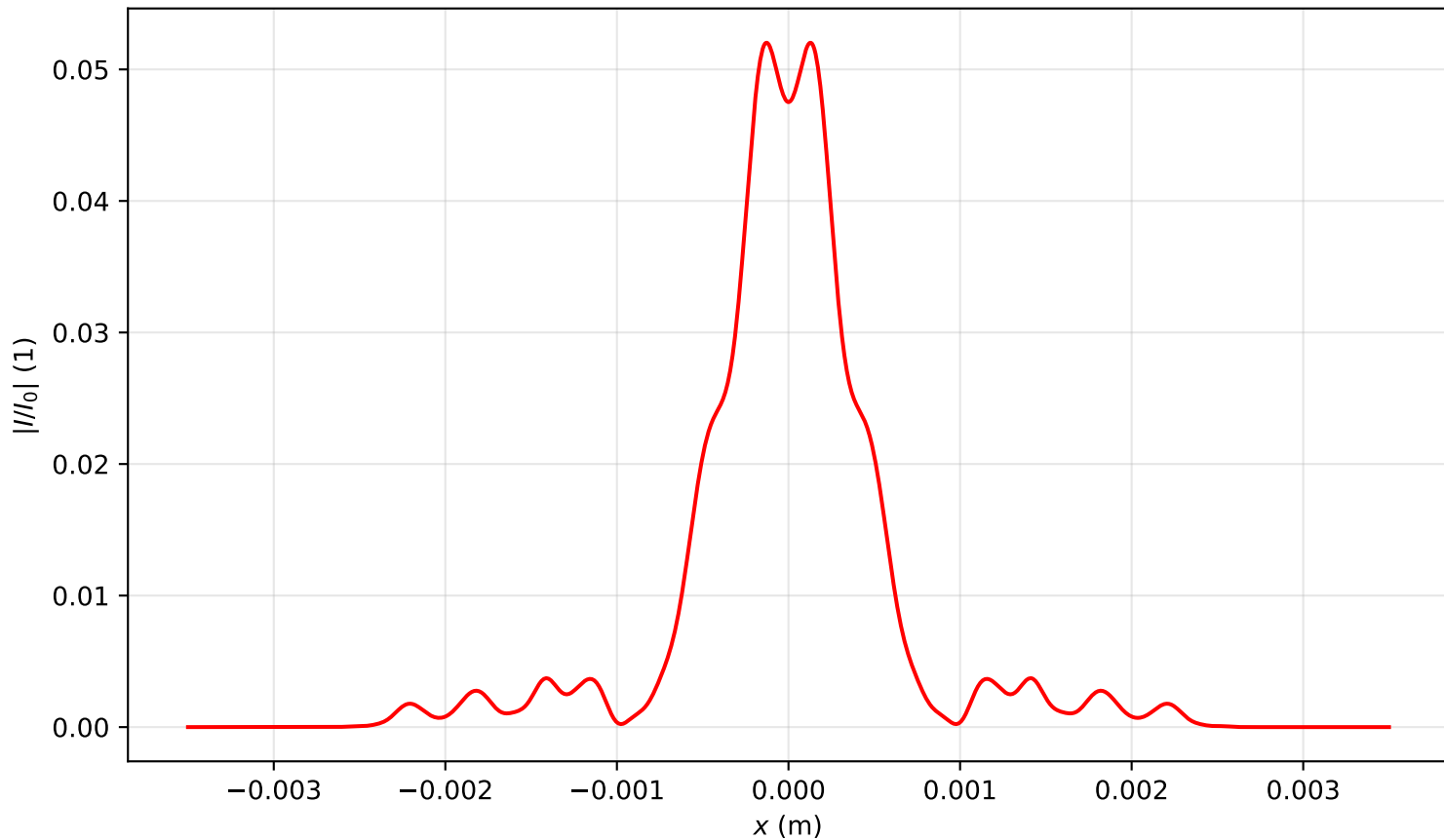
Intensity profile I(x, y = 0, z = 2.388)/I_0 , P_{in}=16.0P_{cr} , artificial time
