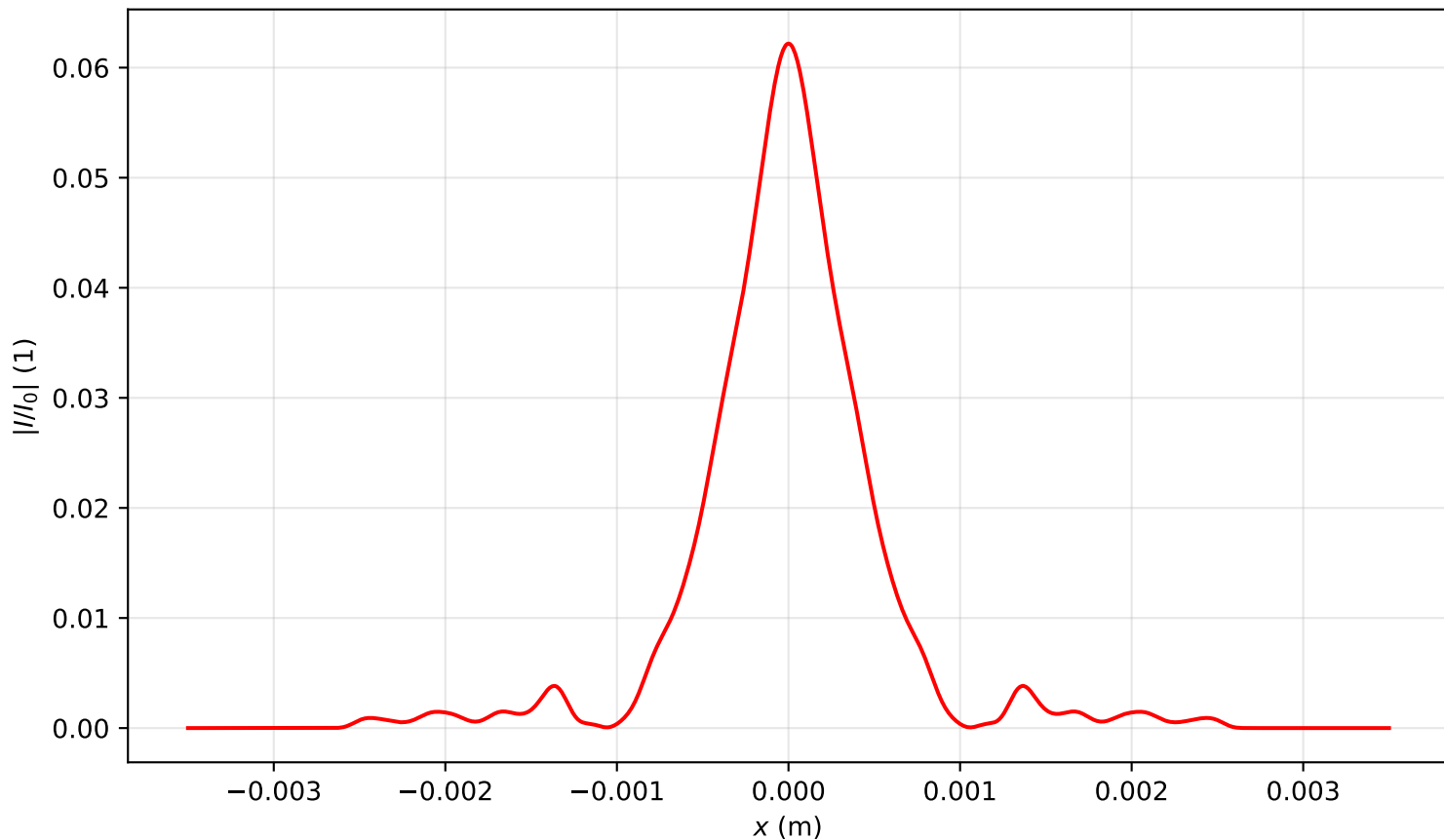
Intensity profile I(x, y = 0, z = 2.548)/I_0 , P_{in}=16.0P_{cr} , artificial time
