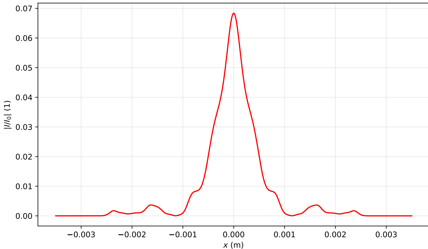
Intensity profile I(x, y = 0, z = 2.707)/I_0 , P_{in}=16.0P_{cr} , artificial time
