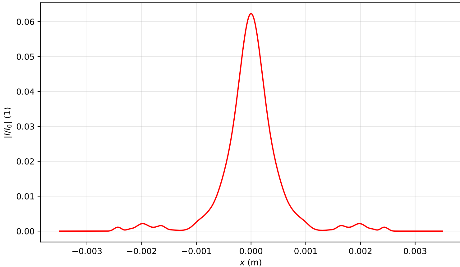
Intensity profile I(x, y = 0, z = 3.025)/I_0 , P_{in}=16.0P_{cr} , artificial time
