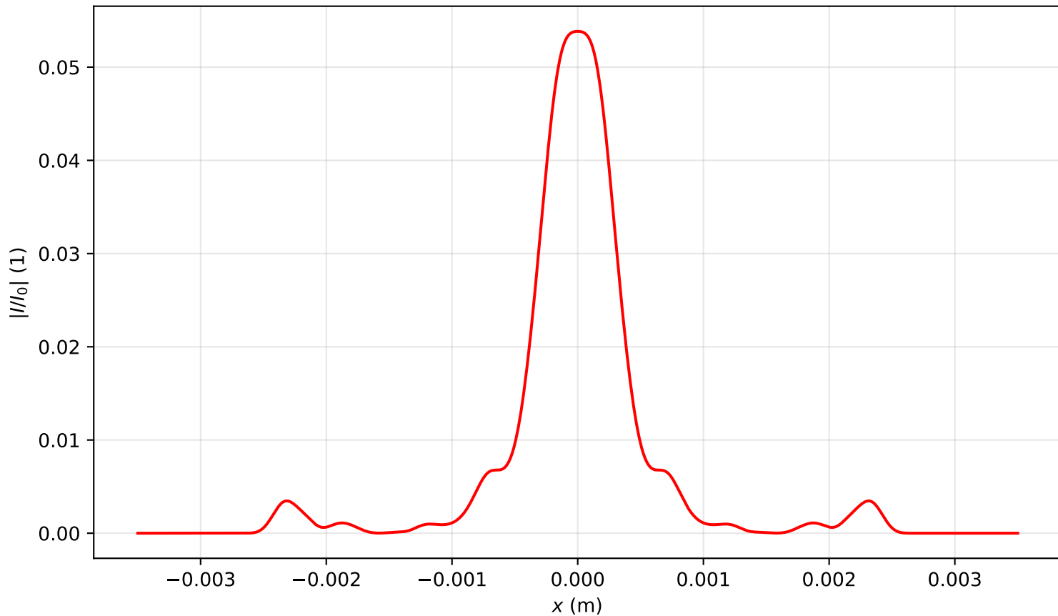
Intensity profile I(x, y = 0, z = 3.503)/I_0 , P_{in}=16.0P_{cr} , artificial time
