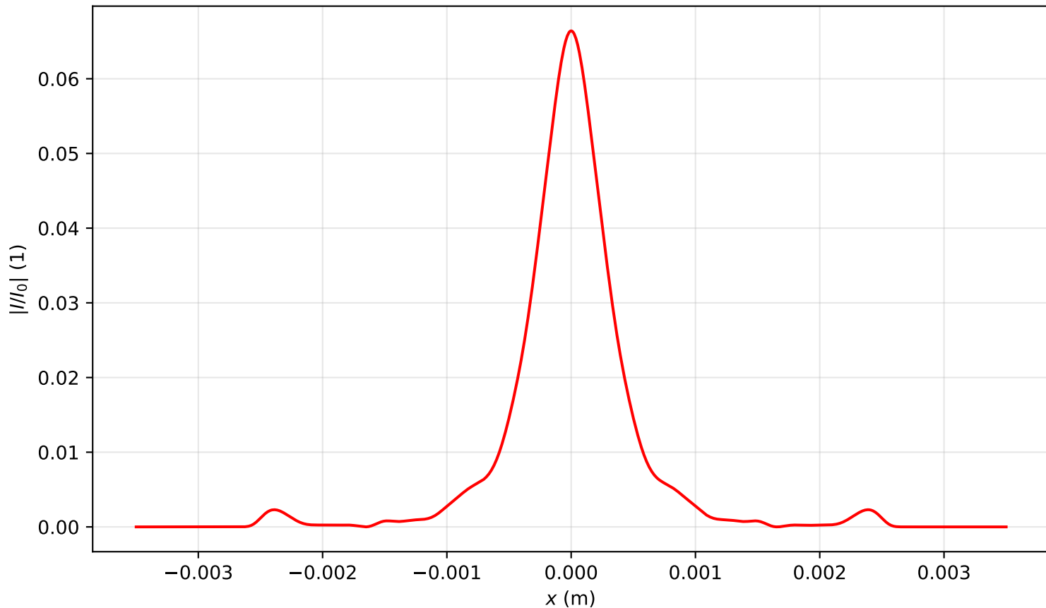
Intensity profile I(x, y = 0, z = 3.662)/I_0 , P_{in}=16.0P_{cr} , artificial time
