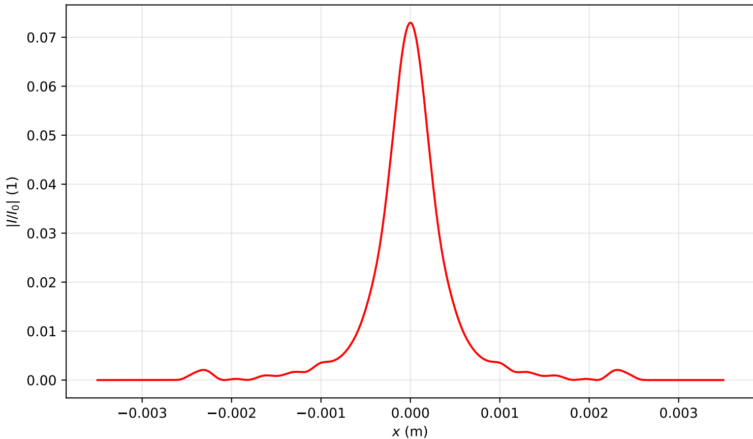
Intensity profile I(x, y = 0, z = 3.981)/I_0 , P_{in}=16.0P_{cr} , artificial time
