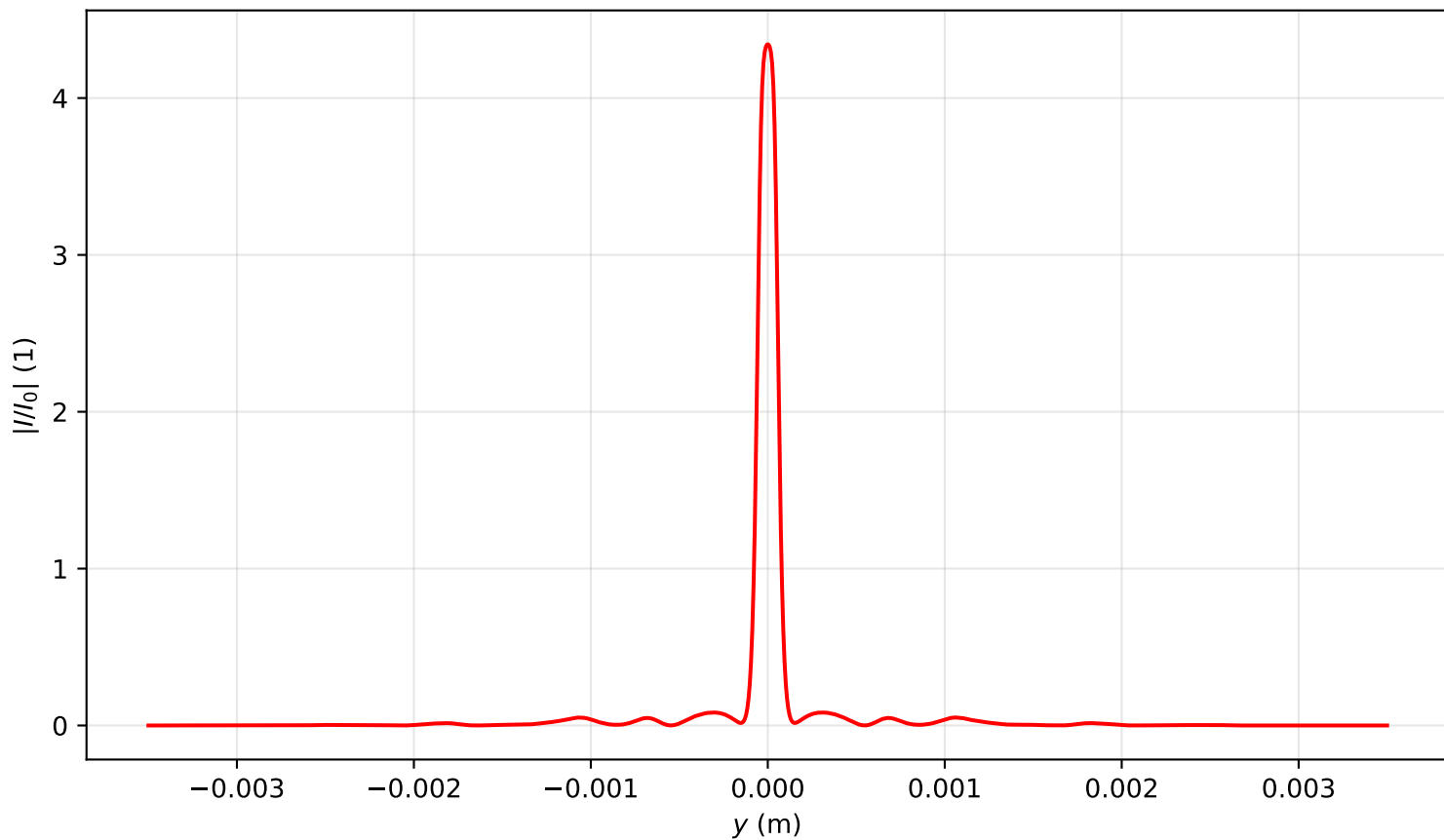
Intensity profile I(x=0, y, z=0.478)/I_0 , P_{in}=16.0P_{cr} , artificial time
