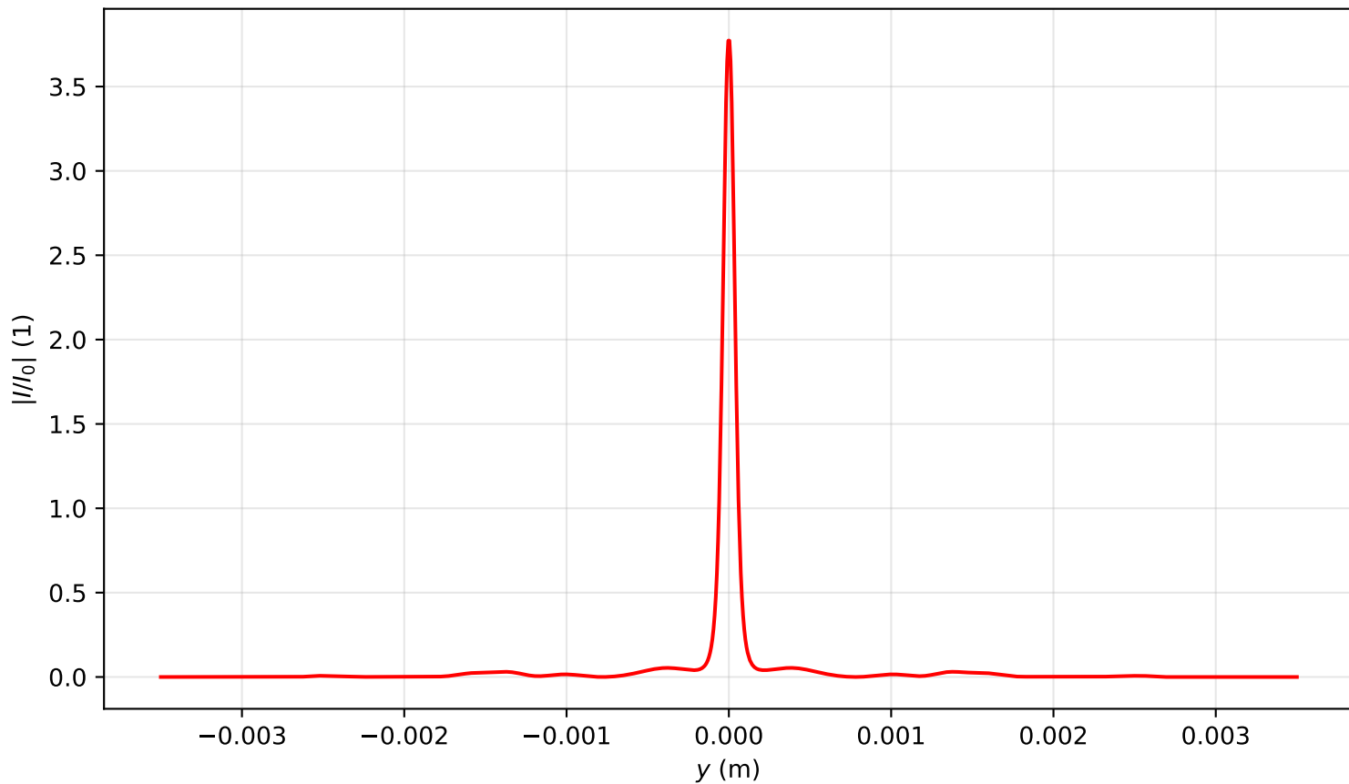
Intensity profile I(x=0, y, z=0.637)/I_0 , P_{in}=16.0P_{cr} , artificial time
