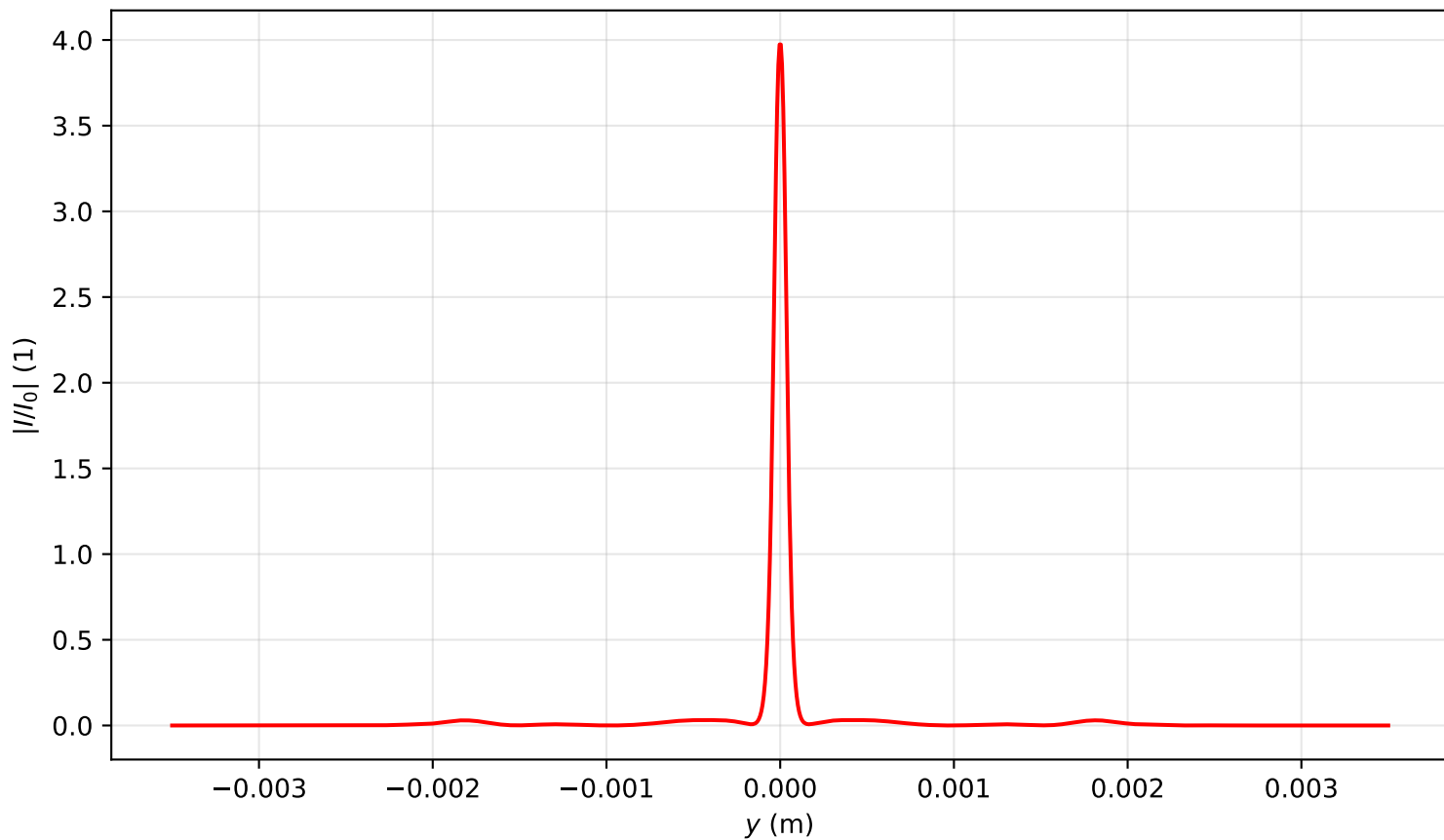
Intensity profile I(x=0, y, z=0.796)/I_0 , P_{in}=16.0P_{cr} , artificial time
