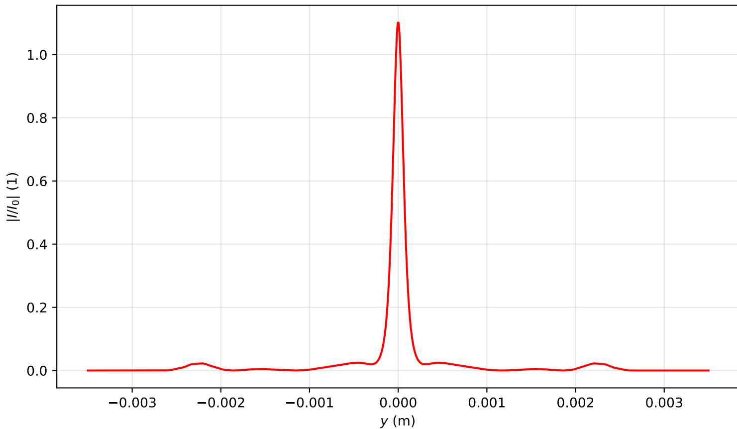
Intensity profile I(x=0, y, z=0.955)/I_0 , P_{in}=16.0P_{cr} , artificial time
