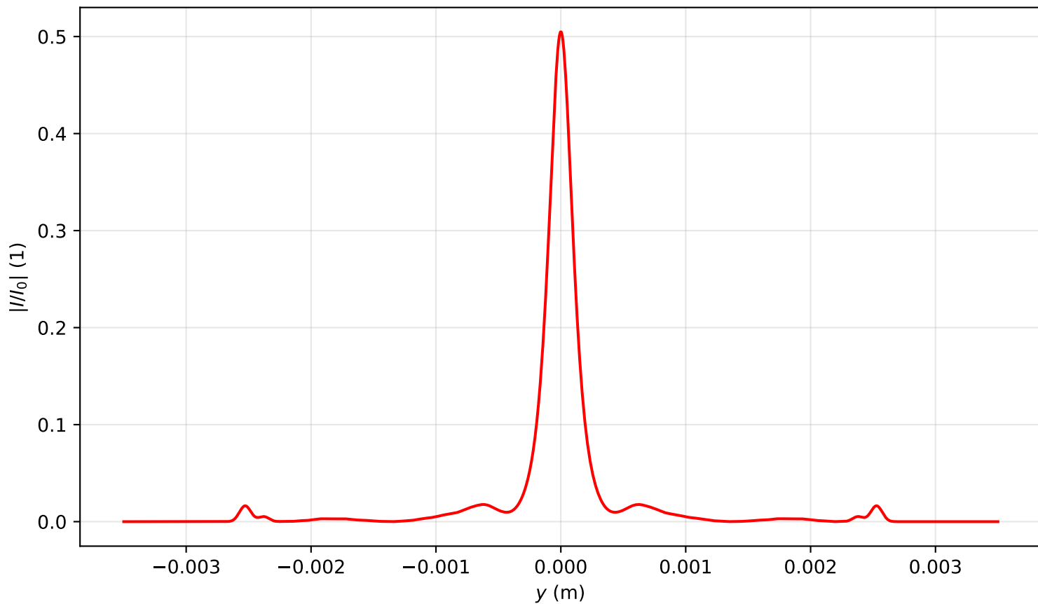
Intensity profile I(x=0, y, z=1.115)/I_0 , P_{in}=16.0P_{cr} , artificial time
