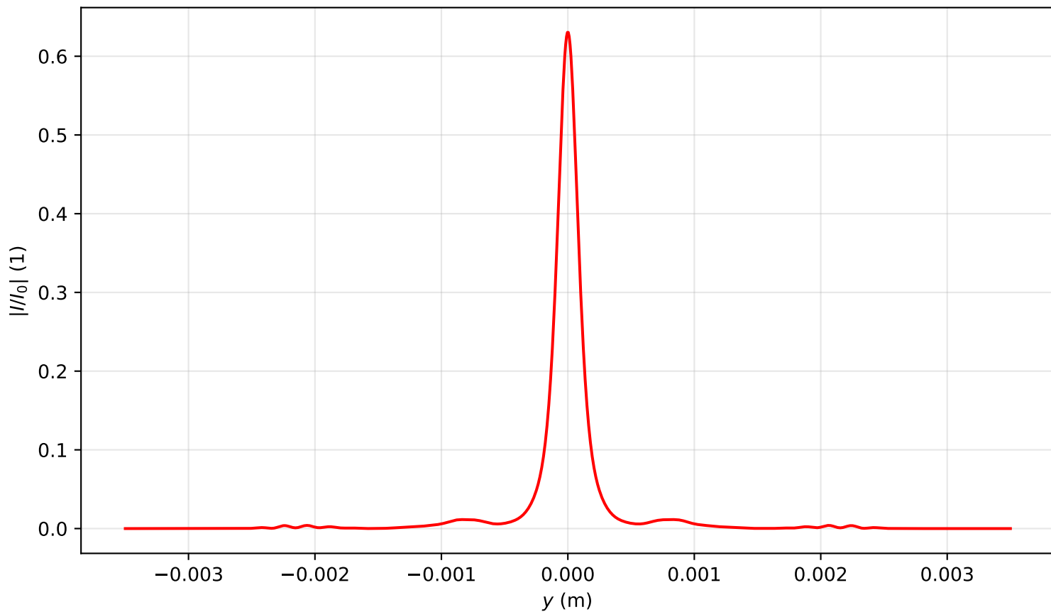
Intensity profile I(x=0, y, z=1.274)/I_0 , P_{in}=16.0P_{cr} , artificial time
