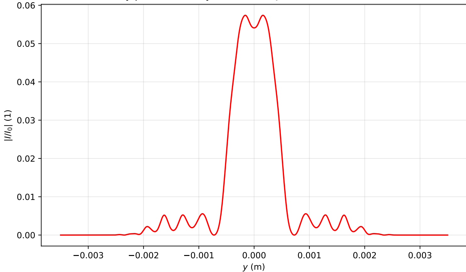
Intensity profile I(x = 0, y, z = 2.070)/I_0 , P_{in}=16.0\text{Pcr} , artificial time
