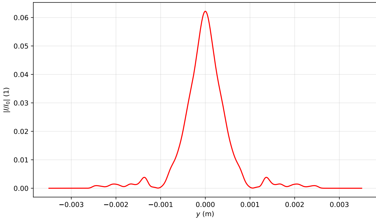
Intensity profile I(x = 0, y, z = 2.548)/I_0 , P_{in}=16.0P_{cr} , artificial time
