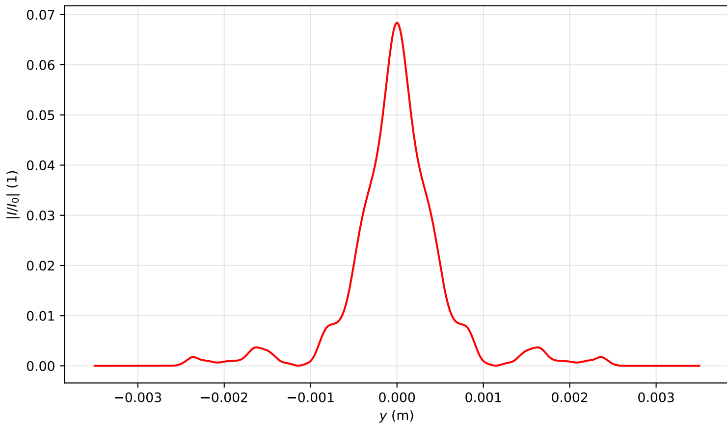
Intensity profile I(x = 0, y, z = 2.707)/I_0 , P_{in}=16.0P_{cr} , artificial time
