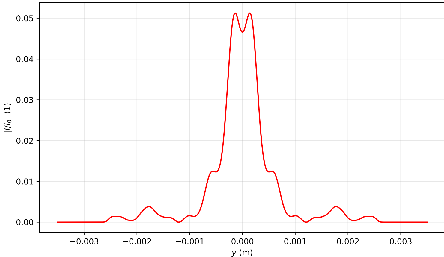
Intensity profile I(x = 0, y, z = 2.866)/I_0 , P_{in}=16.0P_{cr} , artificial time
